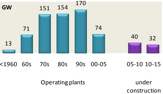
FIGURE 62: DISTRIBUTION OF GAS AND COAL PLANTS
