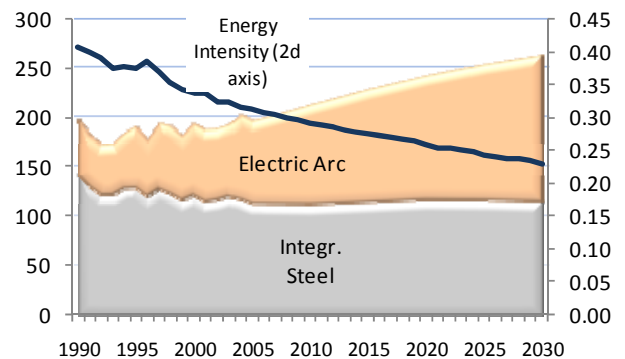
FIGURE 24: IRON AND STEEL SECTOR PRODUCTION (M TONS)
