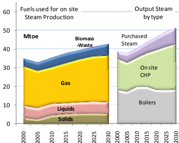
FIGURE 35: STEAM PRODUCTION IN OTHER INDUSTRIES
